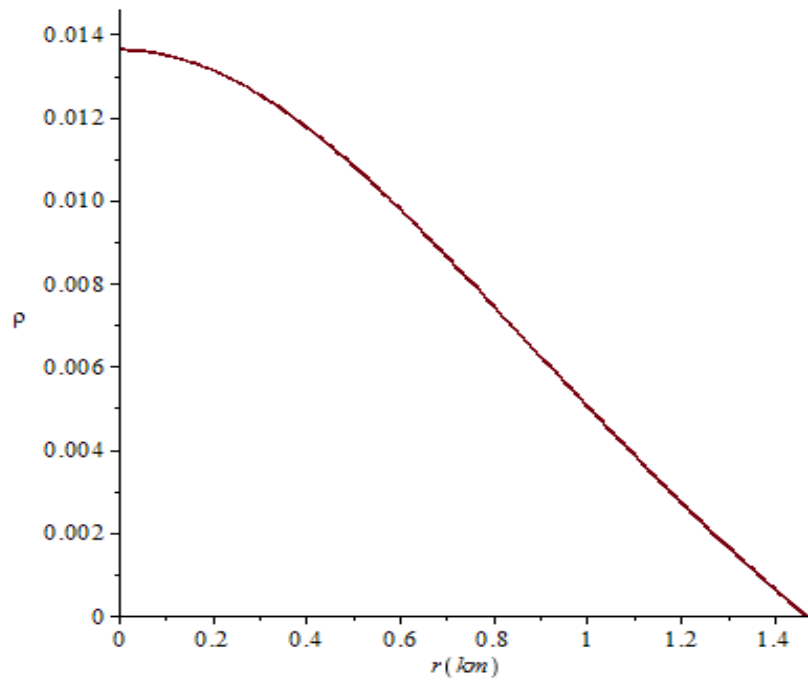
Figure 2. Energy density
