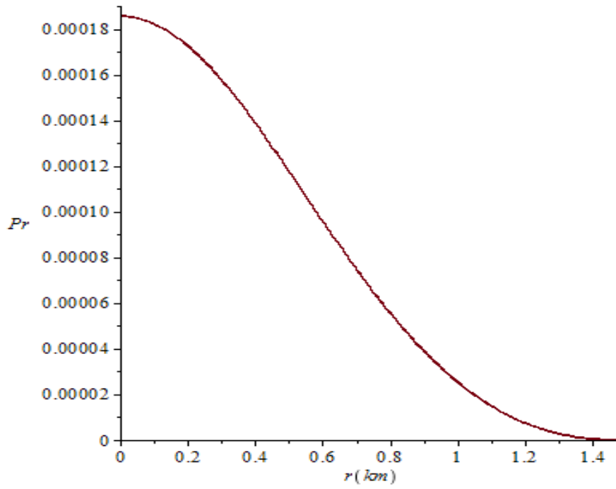
Figure 1. Radial pressure.
