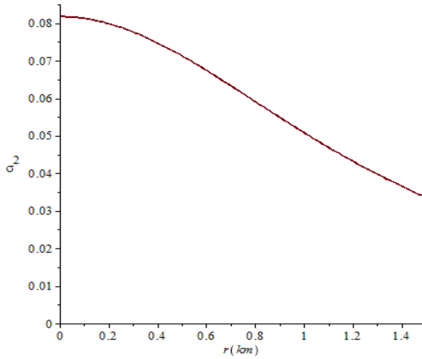
Figure 3. Charge density.
