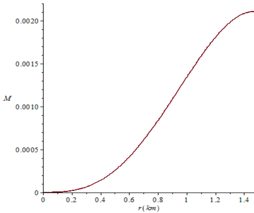
Figure 4. Mass.
