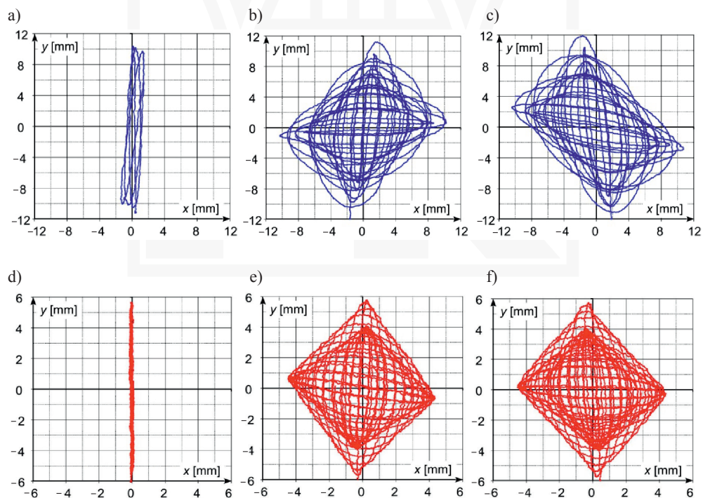
Fig. 7. The trajectory of vibrations at the end of the wire at step reduction of the loading force: a–c) wire Djp100 respectively in normal position (a), rotated by 45^\circ (b), rotated by -45^\circ (c); d–f) wire Djp150 respectively in the normal position (d), rotated by 45^\circ (e), rotated by -45^\circ (f)
