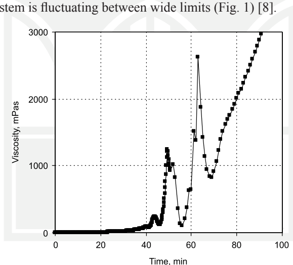
Fig. 1. Transient, induction period of gelation in modified silicate systems [8]
