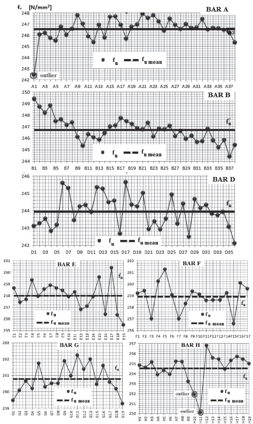
Fig. 6. The sparklines for ultimate strength – E, F, G, H bars
