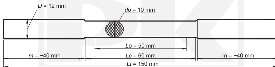
Fig. 2. The proportional round specimen
