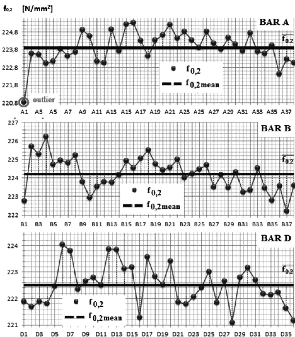
Fig. 4. The sparklines for yield strength – A, B, D bars
