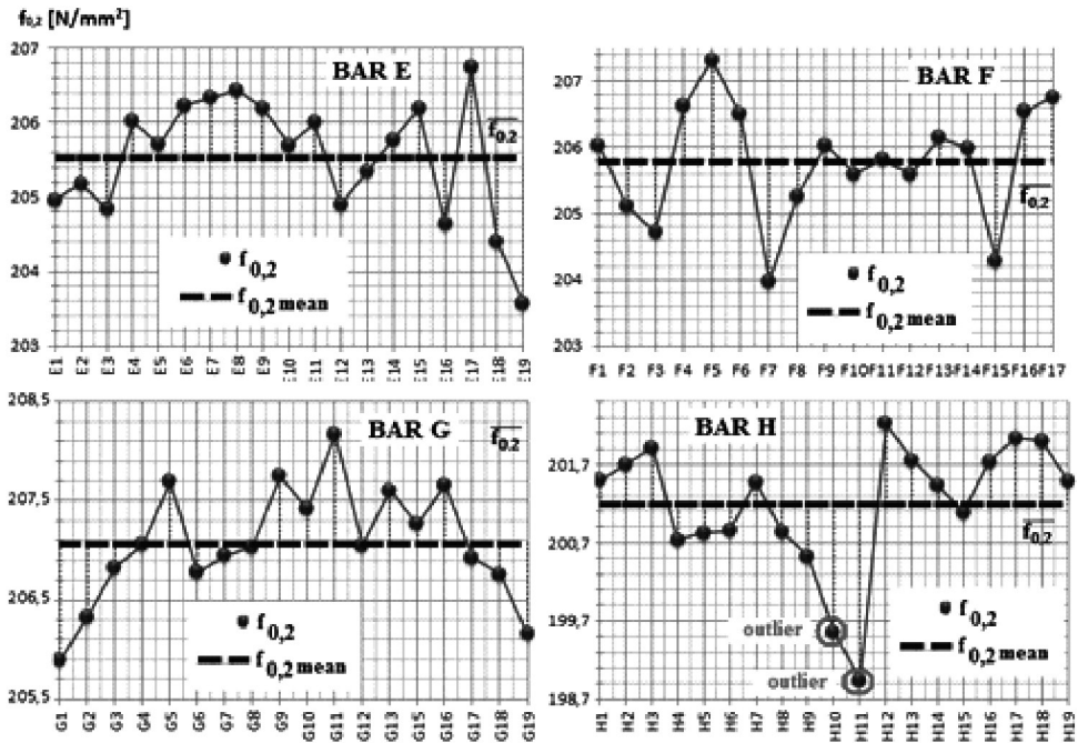
Fig. 5. The sparklines for yield strength – E, F, G, H bars
