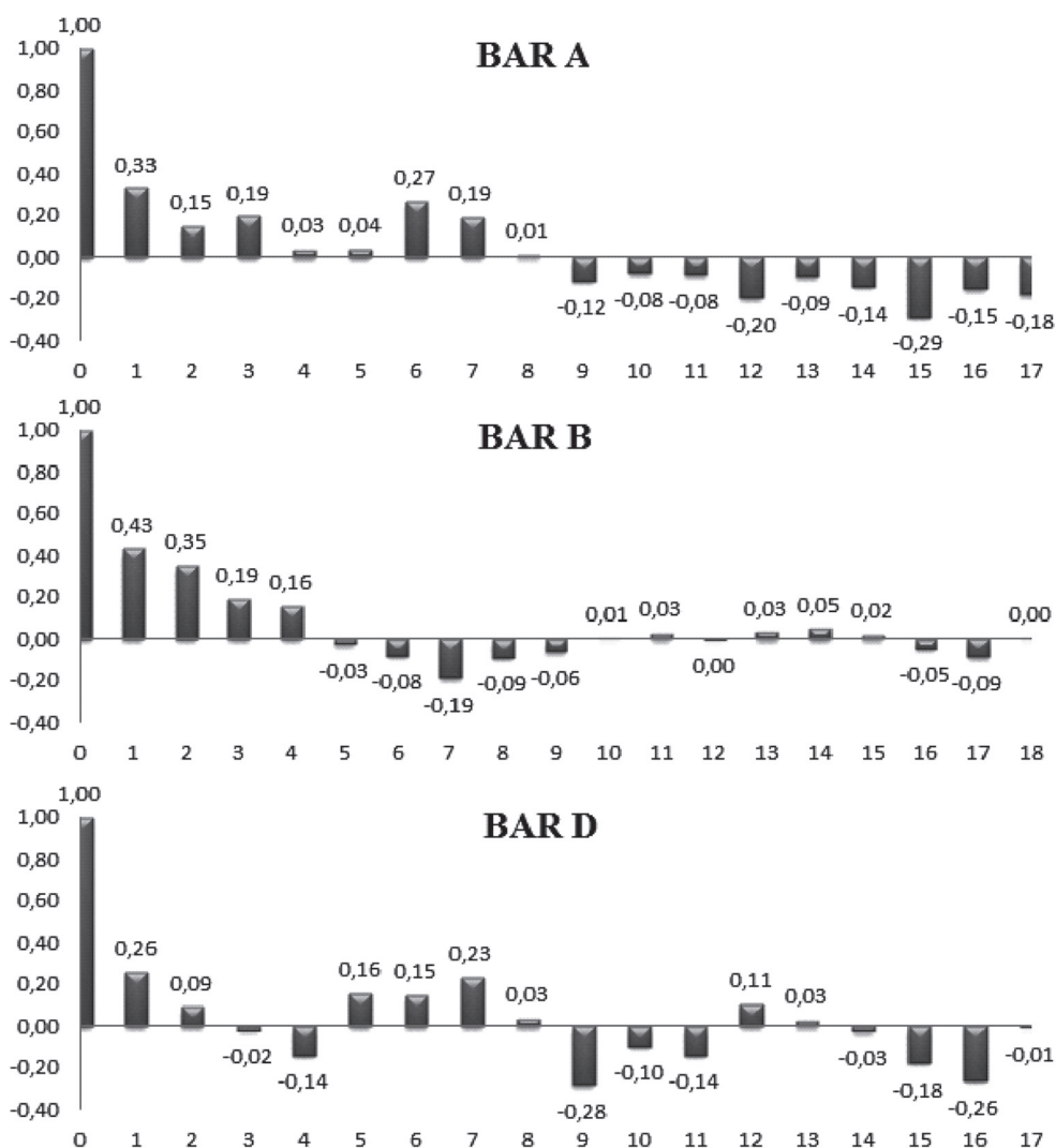
Fig. 8. Autocorrelation function graph for the yield strength
