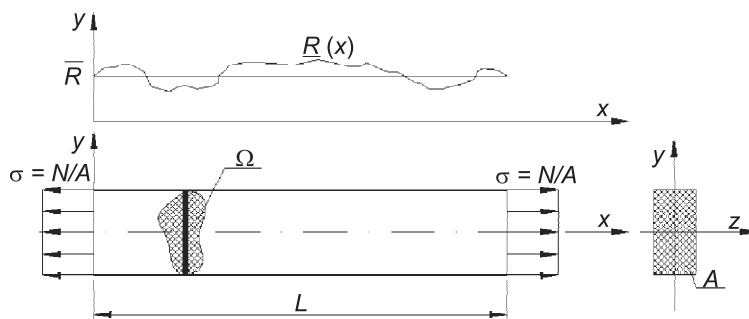
Fig. 1. The concept continual model of bar tensile strength (source: [3] fig. 4.16)
