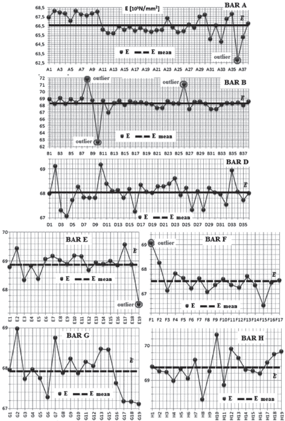
Fig. 7. The sparklines for Young's modulus E – E, F, G, H bars
