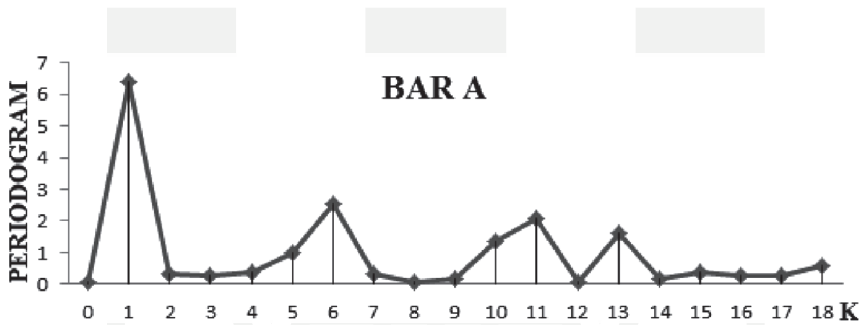
Fig. 10. Periodogram for yield strength
