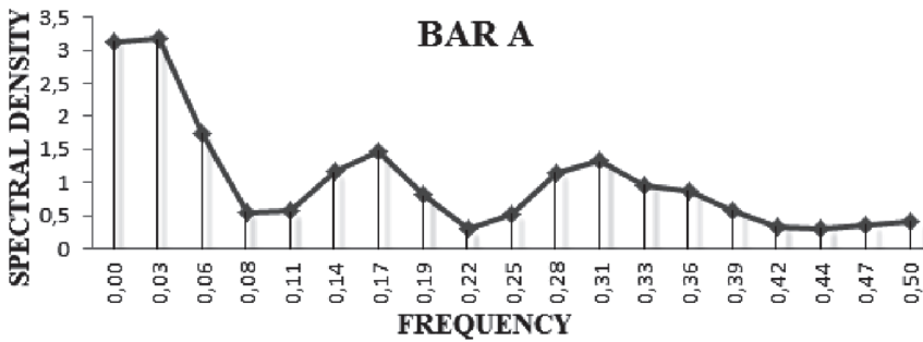
Fig. 9. Spectral density graph for yield strength
