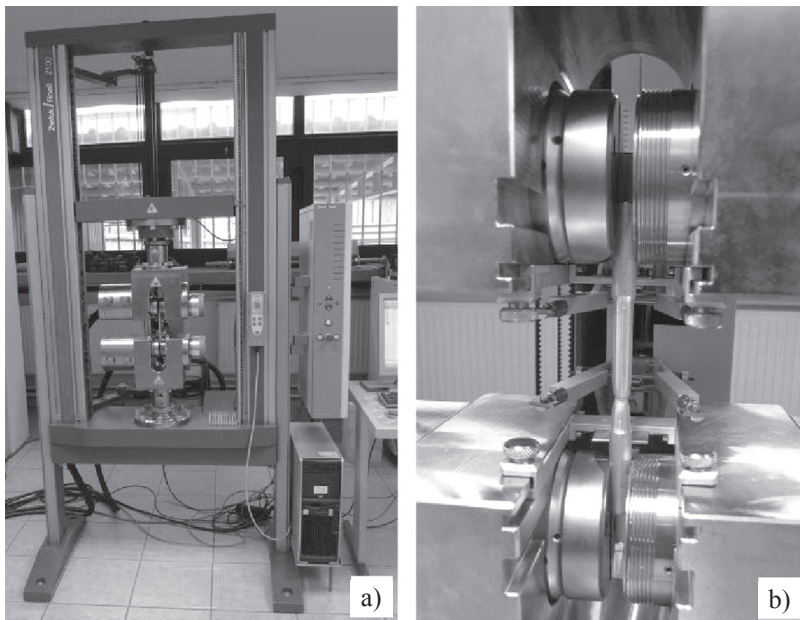
Fig. 3. The static tensile test: a) the testing machine Zwick Roell Z100, b) proper placement of the specimen in the grips (source: [11])
