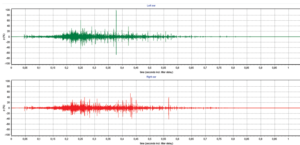
Fig. 5. Impulse response for left and right auditory channels determined at point P1 of the tested hall [9]
