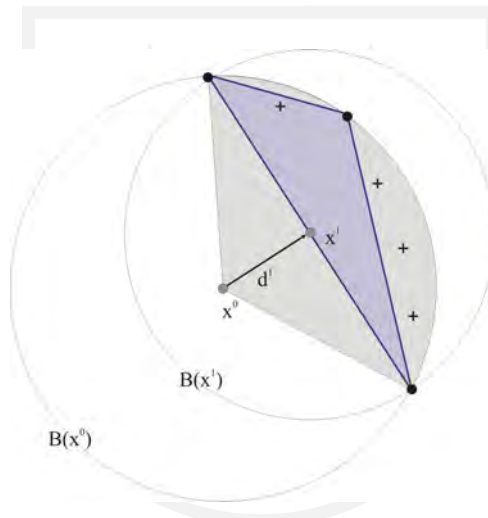
Figure 2. Illustration of the case J^k = \emptyset
