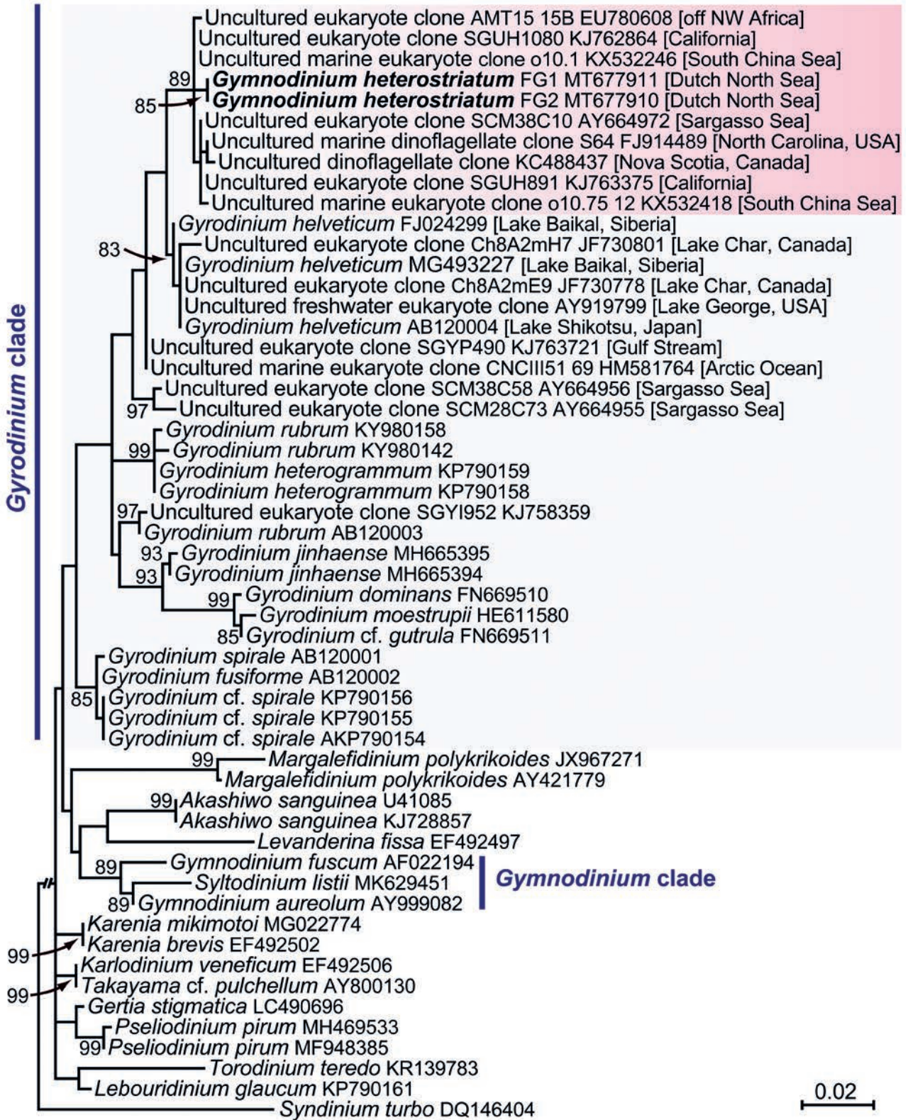
Fig. 3. Phylogenetic tree based on SSU rRNA gene sequences, showing the position of the sequences of Gymnodinium heterostriatum/ striatissimum by Maximum Likelihood (ML). The new sequences are indicated in bold face. Numbers near branches denote ML bootstrap probability value. Bootstrap values <70 are omitted. The geographic origin is placed between brackets. Scale bar denotes 0.02 substitutions per site.
