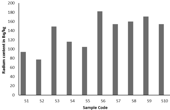
Fig. 4. Results of radium content in the soil samples under study
