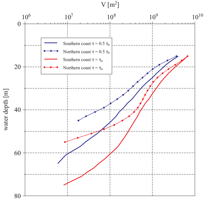
Figure 8. The volumes of water transported to the upper 10-m layer within the Gulf during the upwelling event along either the northern or the southern coast of the Gulf with wind stress \tau = \tau_0 and \tau = 0.5 \tau_0 by day 6 of simulation
