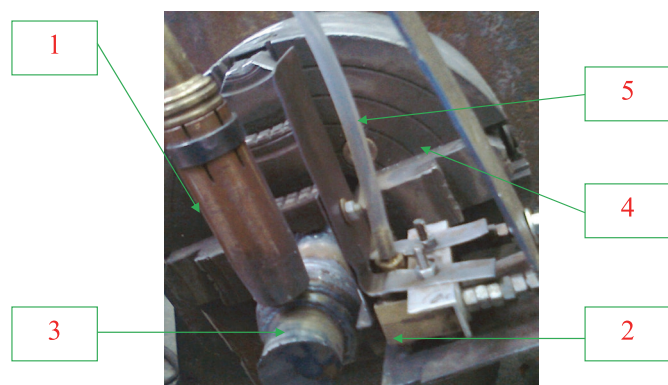
Fig. 1. Position for superficial welding with micro-jet cooling: 1 welding head, 2 micro-jet cooling pipe injector, 3 weld overlay machine shaft, 4 handle, 5 micro-jet gas pipe [21]
