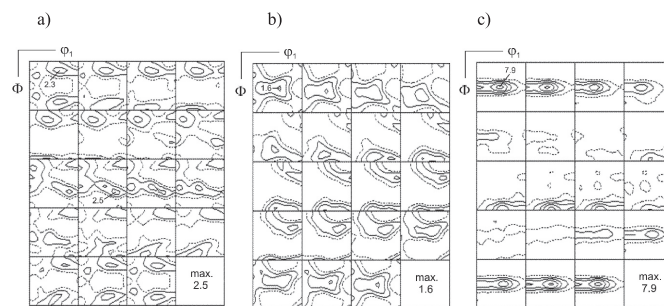
Fig. 10. Experimental orientation distribution functions (ODF's) for (a) \alpha' martensite after 40% deformation, (b) for austenite which was transformed with \alpha' to \gamma according relation K-S and (c) for austenite after 40% deformation
