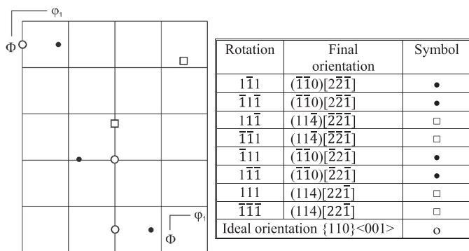
Fig. 8. Transformation of the ideal \{110\} \langle 001 \rangle orientation in the austenite texture according to (2n-1) \times 60^\circ \langle 111 \rangle rotation (section \phi_2=0^\circ ).
