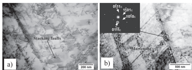
Fig. 2. TEM micrographs of Fe-23Mn-3Si-3Al alloy after 5% cold-rolling and SADPs taken from areas indicated by a circle (a) BF, (b) BF, diffraction pattern [1\bar{1}\bar{1}]_{\epsilon}
