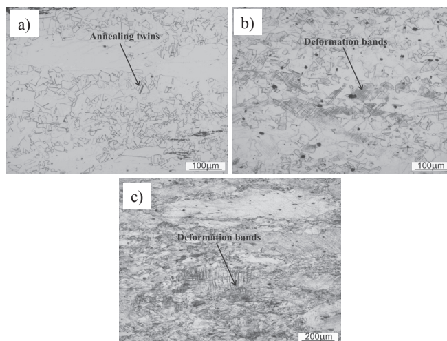
Fig. 1. Microstructure of Fe-23Mn-3Si-3Al alloy (a) in the initial state, after deformation (b) 5%, (c) 30% - light microscopy
