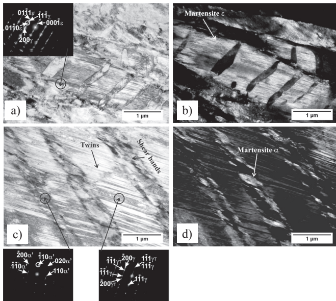
Fig. 3 TEM micrographs of Fe-23Mn-3Si-3Al alloy after 20% cold-rolling and SADPs taken from areas indicated by a circle (a) BF, diffraction patterns [2\bar{1}0]_{\varepsilon} \parallel [011]_{\gamma} , (b) DF with (01\bar{0})_{\varepsilon} , (c) BF, diffraction patterns [001]_{\alpha'} and [011]_{\gamma} \parallel [011]_{\tau} , (d) DF with (\bar{1}10)_{\alpha'}
