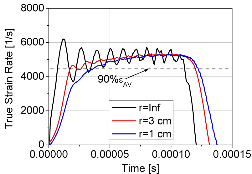
Fig. 11. Influence of striker geometry on true strain rate curve.
