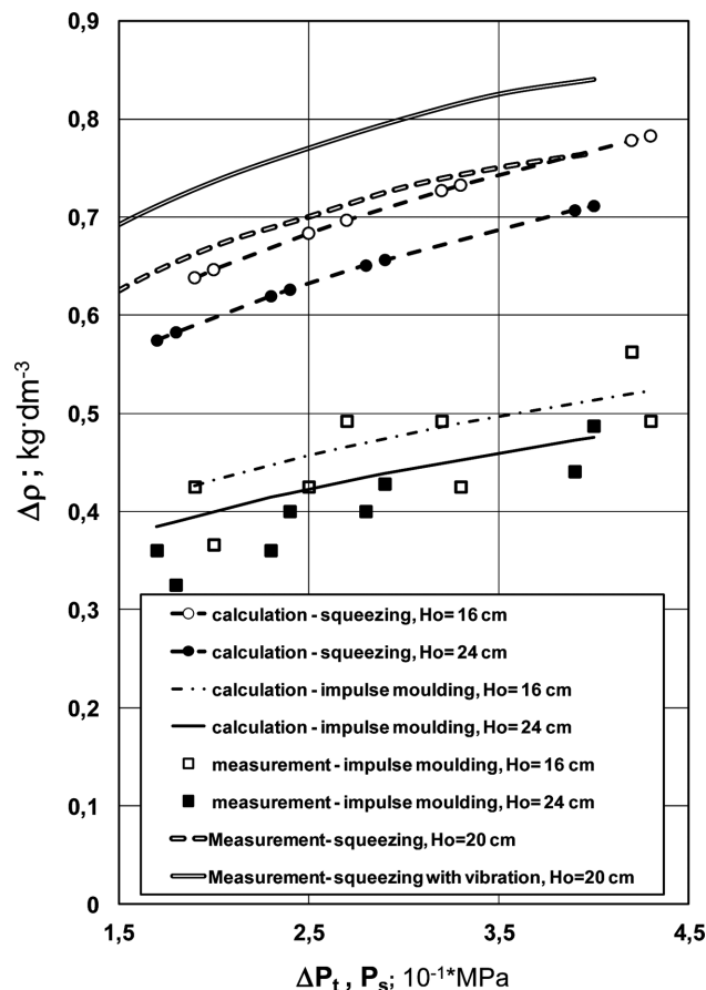
Fig. 2. Dependence between increment of mean mould density – \Delta\rho and maximal overpressure value – \Delta P_t (at impulse moulding) or squeezing pressure- P_s (at squeezing): initial height of moulding sand layer H_0 = 16 cm- \rho_0 \approx 0.94 kg/dm^3 , initial height of moulding sand layer H_0 = 24 cm- \rho_0 \approx 0.97 kg/dm^3 . Calculation acc. eq. (1) at k=0,2 for impulse moulding and k=1 for static squeezing. Measurement data for squeezing and squeezing with vibration from [5]
