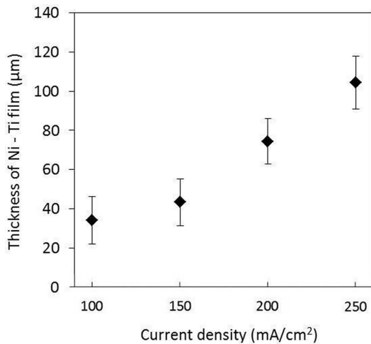
Fig. 3. Thickness as a function of current density with a Ti-particle loading of 8 g/dm 3
