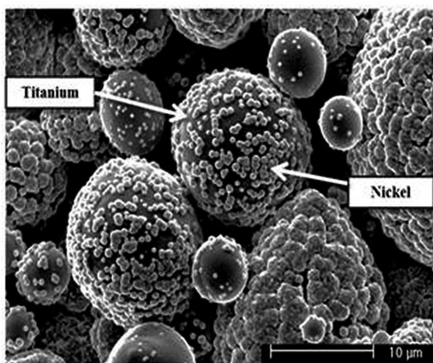
Fig. 11. Microstructure of the Ni-Ti composite coating illustrating the preferential Ni deposits on Ti particle surfaces
