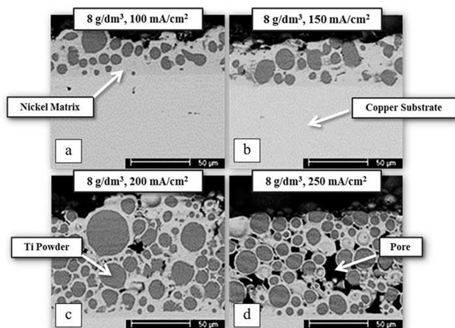
Fig. 9. Cross-sectional images (Back-scattered electron mode) of the Ni-Ti composite coatings deposited with the particle loading of 8 g/dm 3 under the following current densities of (a) 100 mA/cm 2 , (b) 150 mA/cm 2 , (c) 200 mA/cm 2 , (d) and 250 mA/cm 2
