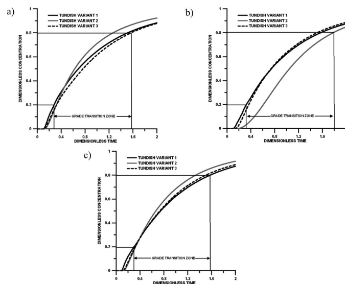
Fig. 5. Grade transition zone characteristic for all variants of present-ed tundish (a) tundish outlet no. 1 (b) tundish outlet no. 2 (c) tundish outlet no. 3
