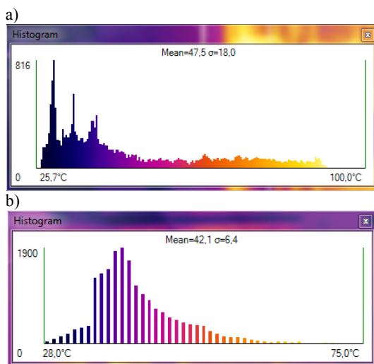
Fig. 6. Histogram of temperature field of area 1 of mold equipment in manufacturing machine: a) No. 1 (Fig.4), b) No. 2 (Fig. 5)
