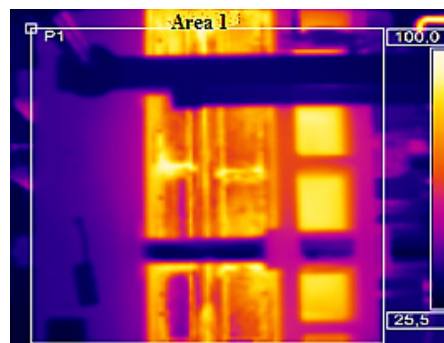
Fig. 4. Temperature field of mold equipment in manufacturing machine No. 1 - view from mold parting side
