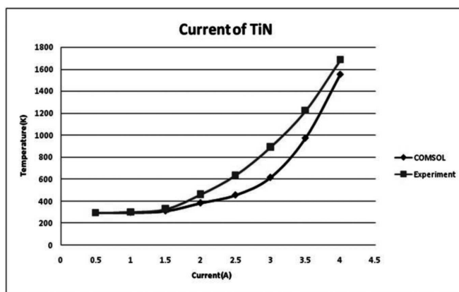
Fig. 7. Current Vs Temperature of 0.075 mm diameter TiN wire element
