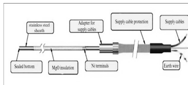
Fig. 1. Components of micro tubular coil heater
