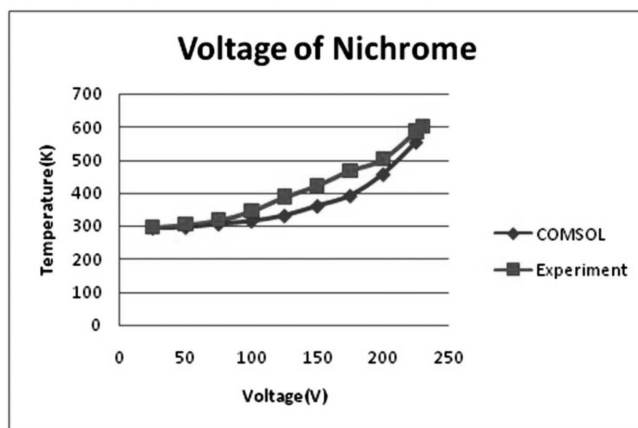
Fig. 8. Voltage Vs Temperature of 0.075 mm diameter Nichrome wire element
