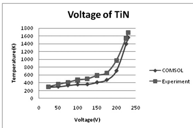
Fig. 9. Voltage Vs Temperature of 0.075 mm diameter TiN wire element
