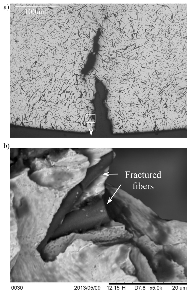
Fig.1 Microstructure of composite materials Cu-10vol. % Saffil fibres after bending test at 20°C. Crack propagated at the side where tension stresses were created (a), fracture with broken fibers in area marked in a subsection (b)
