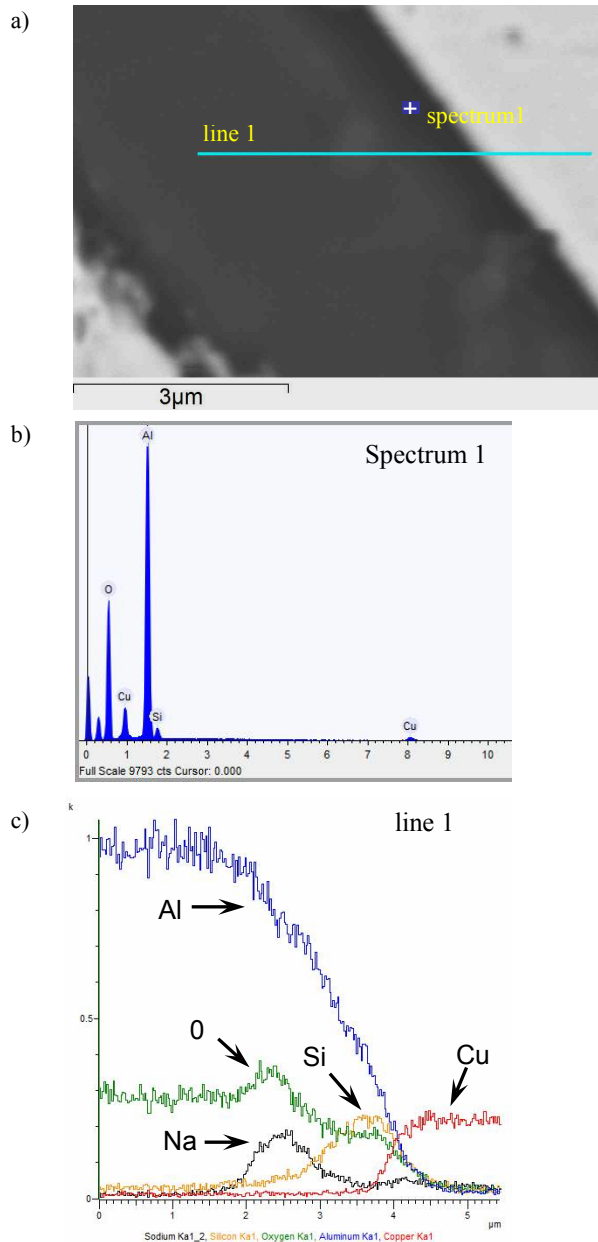
Fig. 5. Fiber-matrix area with marked point and line of EDS analysis (a), point analysis of the interface (b), line distribution of Al, O, Si, Na and Cu elements (c)
