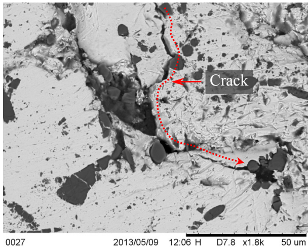
Fig.3. Microstructure of composite material Cu-10 vol.% Saffil after bending in fractured region with propagation of crack thorough Cu matrix between \text{Al}_2\text{O}_3 fibres.
