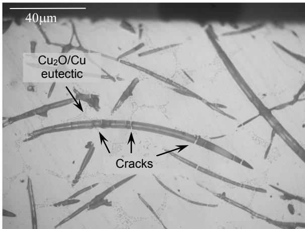
Fig.2. Microstructure of Cu-10 vol.% Saffil fibres composite materials examined at 300°C with fragmented fibres subjected to tension stresses.
