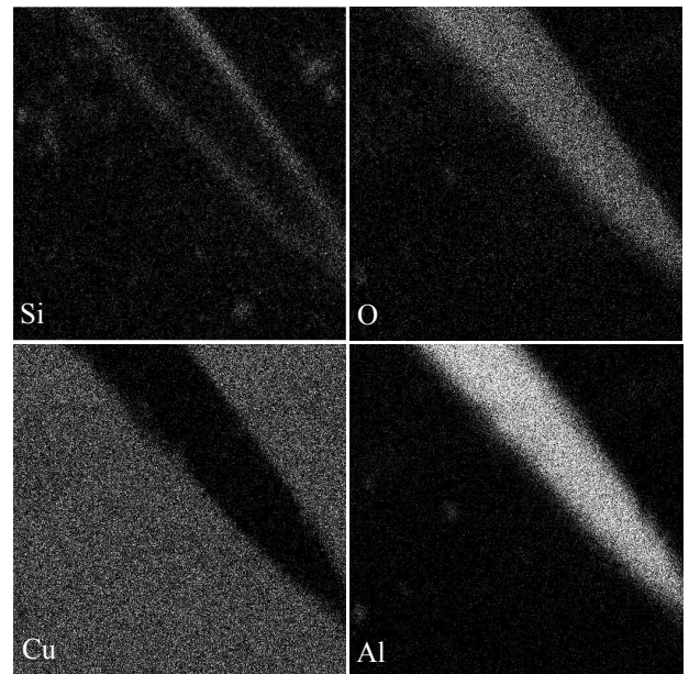
Fig. 4. Alumina fiber embedded in Cu matrix with mapping of Si, O, Cu and Al and elements
