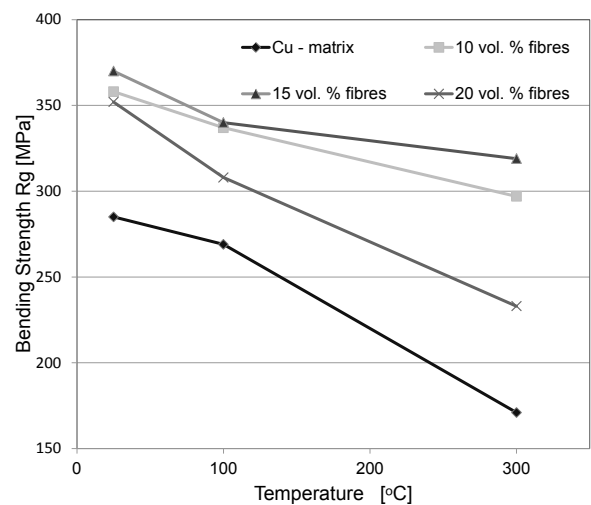
Fig. 6. Bending strength of unreinforced and copper based composite materials strengthened with 10, 15 and 20% of alumina fibers.
