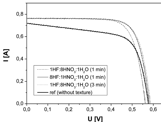
Fig. 7. Current-voltage characteristics of 25 cm 2 mc-Si solar cells depending on mixture content and time of texturization process
