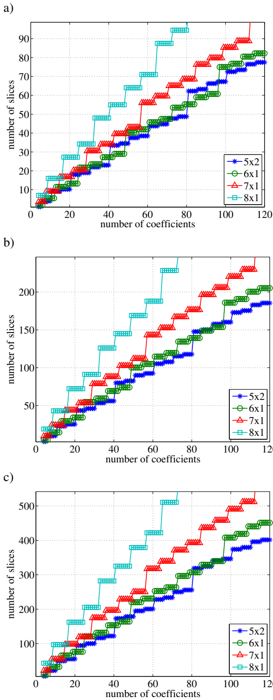
Fig. 4. The estimation of utilized Xilinx Virtex-5 and Virtex-6 FPGA resources after decomposition of DA-LUT block using dual adders, depending on number of coefficients, and type of logic cells, for various coefficients bit width a) 4 bits b) 16 bits c) 40 bits .
