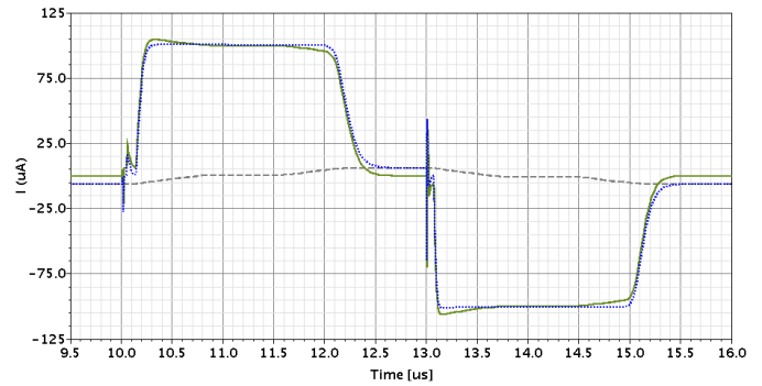
Fig. 11. Currents related to output stage of the circuit without voltage buffer: current flow from the generator (dotted), current flow to the output capacitor (solid), current flow to the edge-rounding circuitry (dashed).
