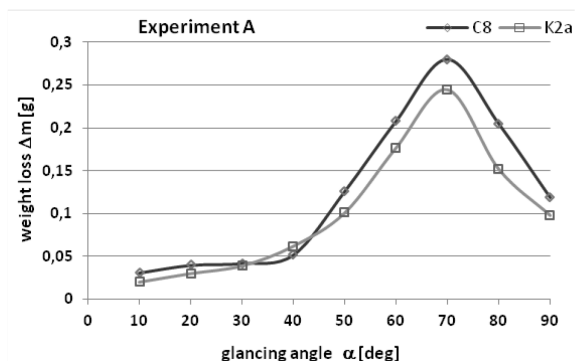
Fig. 7. Wear abrasive of low-alloyed cast steel (K2a) and steel (C8) in the function of the angle of incidence of quartz sand on the surface of measuring specimens
