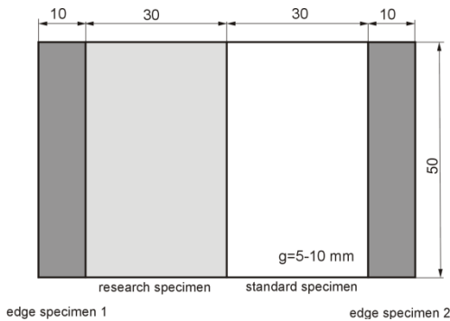
Fig. 3. Set of specimens fixed in the holder
