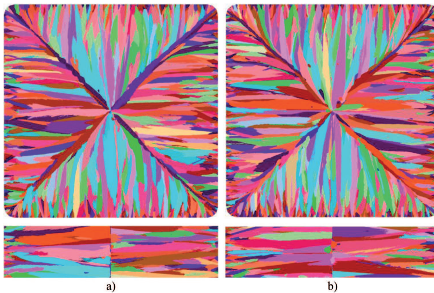
Fig. 5. Primary grains' structure of the S235JR (a) and B500 SP (b) steel in the cross and longitudinal sections of the continuous strands of size 160×160 mm (modeling)
