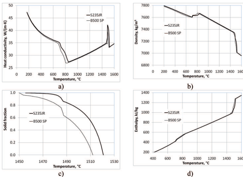
Fig. 3. Temperature dependence of the heat conductivity (a), density (b), solid fraction (c) and enthalpy used in the simulation
