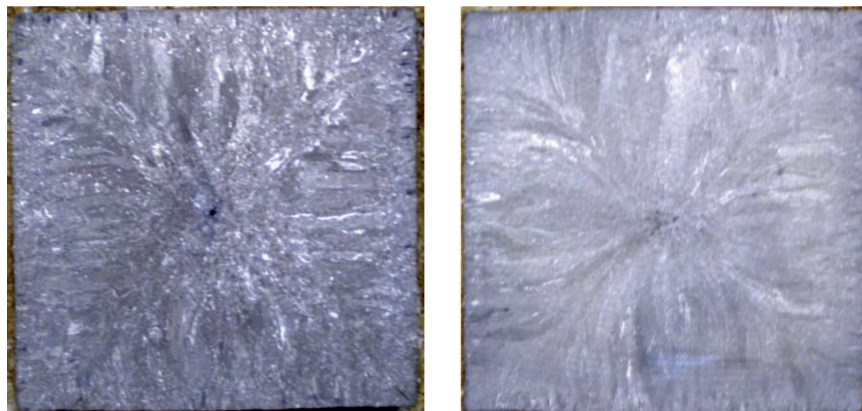
Fig. 6. The samples of the cross section structure in the continuous ingot of size 160×160 mm. Steel grade S235JR (PN-EN 125-2)
