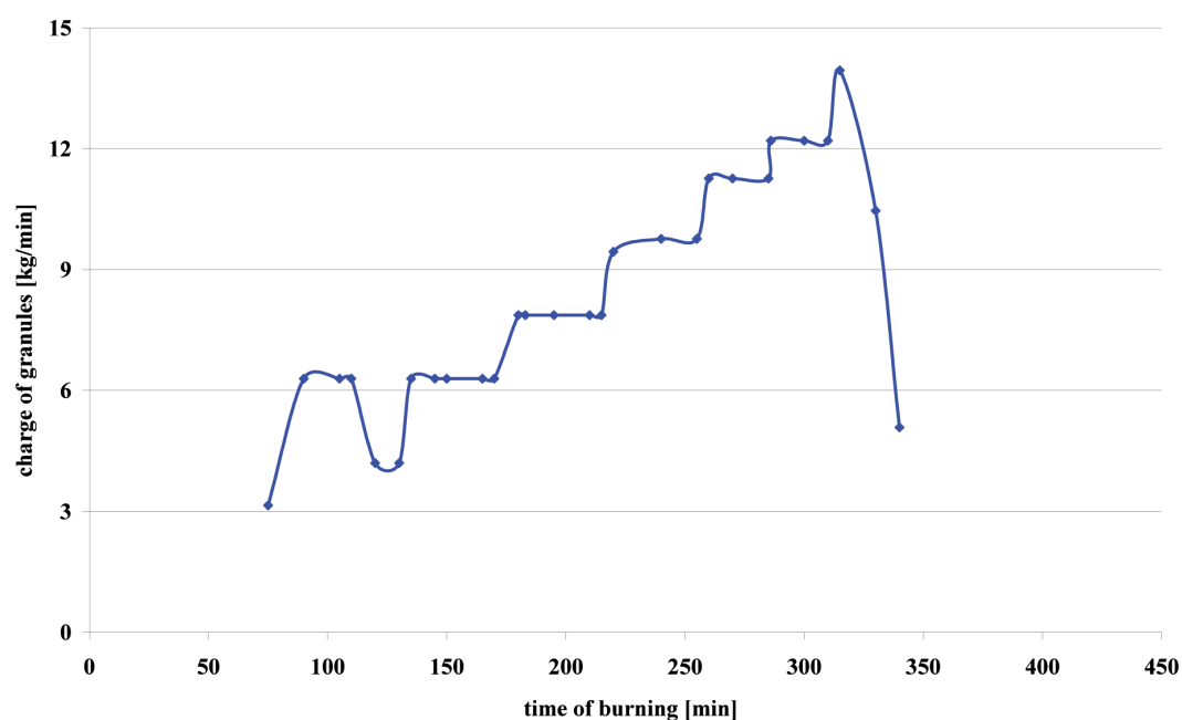
Fig. 9. Flux of granules delivered to the furnace
