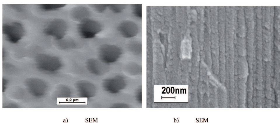
Fig. 1. Surface view (a) and fracture (b) from anodic hard coating used as matrix of composite layer AHC+GC, nanopores as dark near circle shaped dots – Fig a – and vertical canals – Fig b
