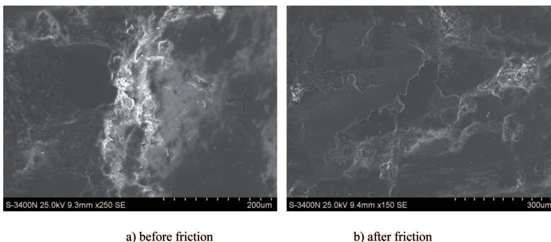
Fig. 6. Big macro-cracks in oxide layer after carbonizing process at higher temperature before (a) and after friction (b: small scratches in friction direction made by sliding cast-iron pin)
