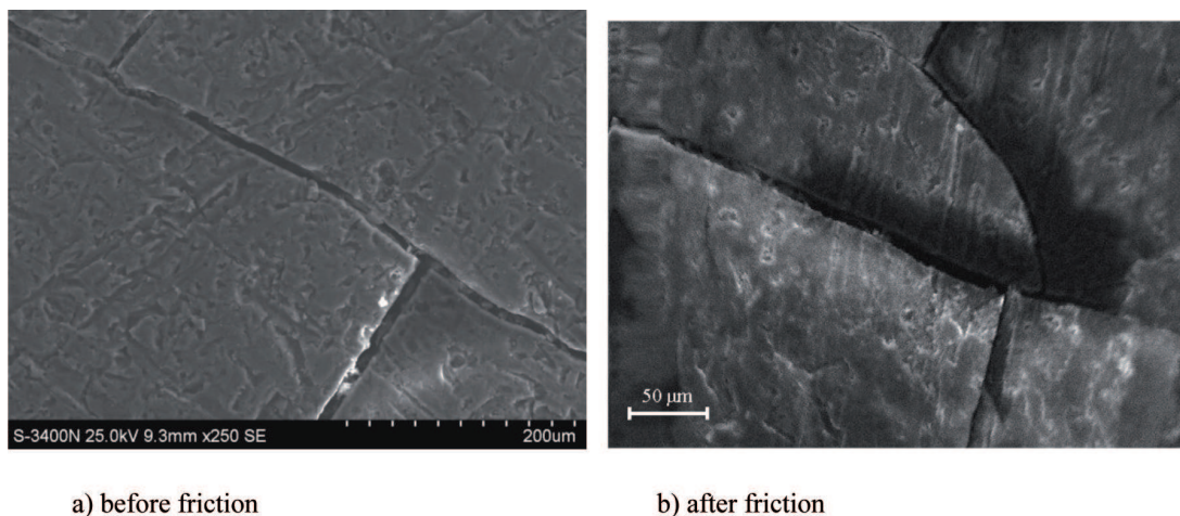
Fig. 5. Small macro-cracks in oxide layer after carbonizing process at lower temperature (a – sharp edges; b – edges smoothed during friction)
