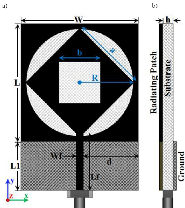
Fig. 1. Geometrical structure of the proposed antenna (a) top view and (b) side view
