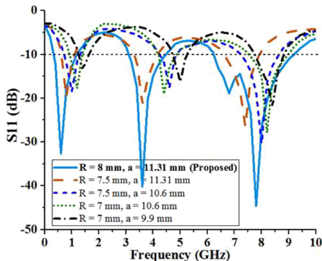
Fig. 4. Effect of varying radius of circle and side length of rhombus on the bandwidth and reflection coefficient (S11)
