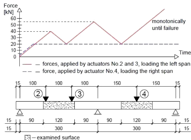
Fig. 8. Variable loading scheme (B) and areas examined with 3D scanner Aramis
