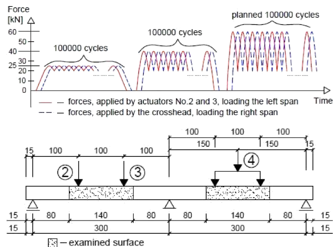
Fig. 10. Variable cyclic loading scheme causing shear failure with areas examined with 3D scanner Aramis
