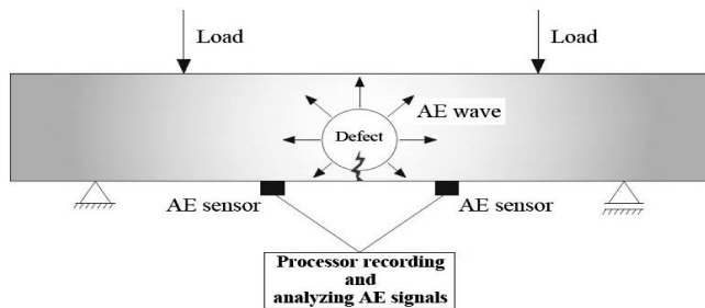
Fig. 1. Diagram of wave generation by destructive processes and wave recording
