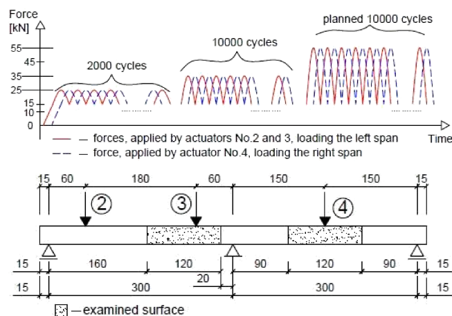
Fig. 9. Cyclic loading scheme (C) and areas examined with 3D scanner Aramis
