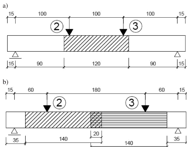
Fig. 6. a) Bending load and area examined with Aramis (one arm), b) shearing load and area examined with Aramis (two arms)
