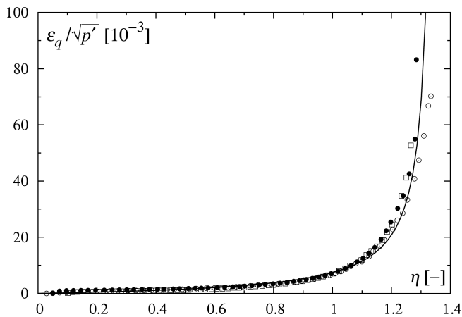
Fig. 6. Deviatoric strains that develop during pure shearing (path ABC in Fig. 4) – a common plot for three experiments performed at different values of the mean effective stress
