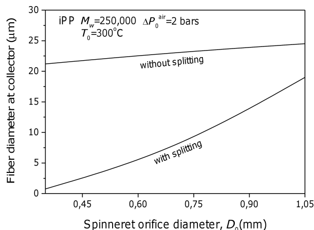
Fig. 9. Diameter of iPP filament on the collector vs. orifice diameter D_0 computed for air compression \Delta P_0^{air} = 2 bars in the process without and with fibrylar splitting. M_w=250,000 , T_0=300^\circ\text{C} , W=0.04\text{g/s} , L=20\text{cm}
