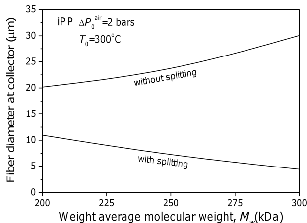
Fig. 6. Diameter of iPP filament at the collector vs. average molecular mass M_w computed for air compression \Delta P_0^{air} = 2 bars in the process without splitting and the diameter of sub-filament in the ideal fibrillar splitting, T_0 = 300^\circ\text{C} , W = 0.04 g/s, D_0 = 0.7 mm, L = 20 cm
