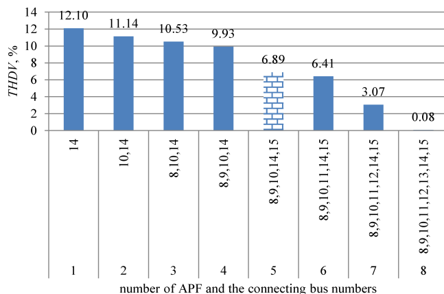
Fig. 6. Comparison of THDV values in the chosen bus of the system for variable number of compensators (from 1 to 8) and different connection arrangements (the numbers of buses are given) – optimization strategy (C)
