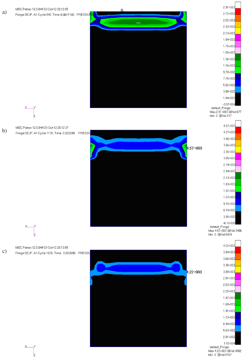
Fig. 12. Propagation of internal membrane pressure wave (caused by the incident pressure impact) for different time steps: a) 0.001718 s, b) 0.002248 s, c) 0.0026865 s
