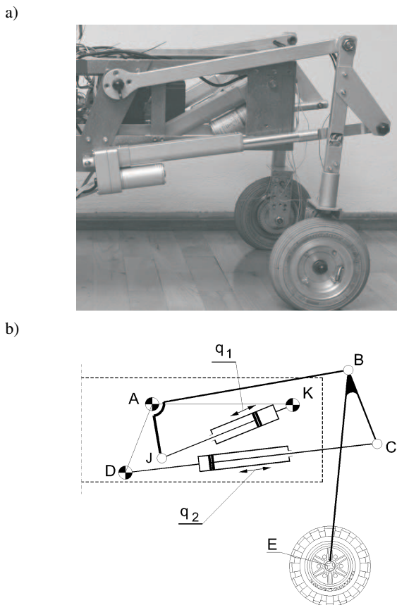
Fig. 2. Robot’s limb: a – general view, b – kinematic scheme
