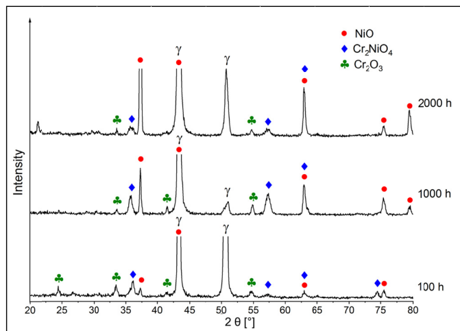
Fig. 3. XRD Bragg-Brentano pattern of the Inconel 686 clad layer after oxidation in waste incineration ashes for 100, 1000 and 2000 h at 650^\circ\text{C}
