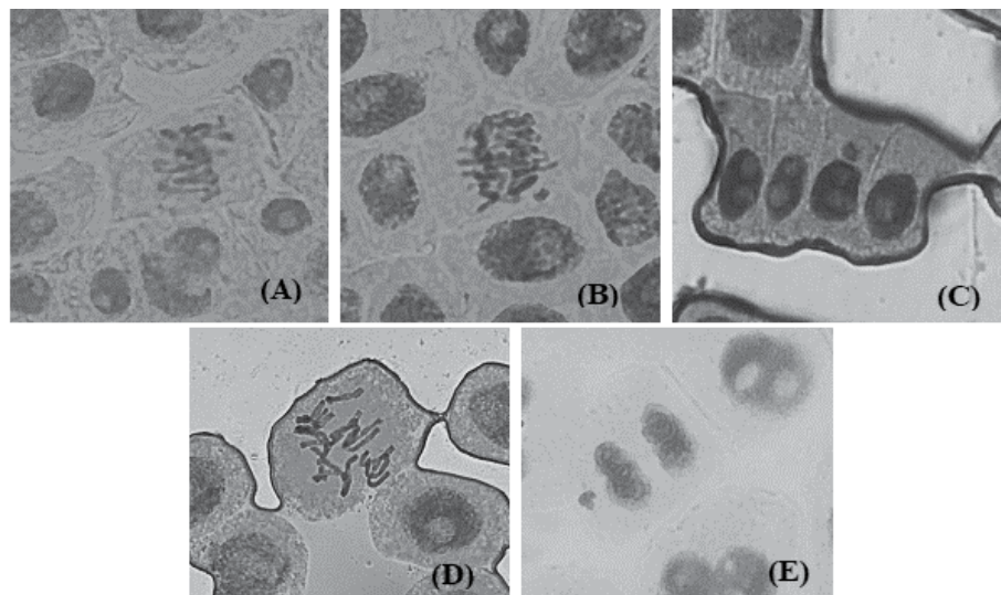
Fig. 3. Mitotic division abnormalities determined in the root tips of A. cepa L. treated with IWW samples (A) Irregular metaphase; (B) Stickiness and fragment; (C) Micronucleus; (D) C-Mitosis; (E) Vagrant Chromosome
