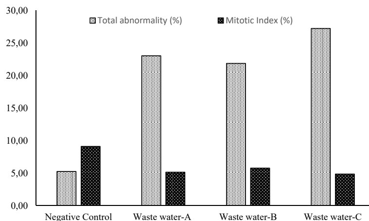
Fig. 4. The relationship between total abnormality (%) and mitotic index (%) in A. cepa treated with IWWs for 48 h ( p \leq 0.001 )
