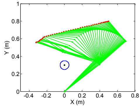
Fig. 14. Series of configuration corresponding to minimum energy motion planning when the singularity avoidance is not considered, however, obstacle avoidance is in force
