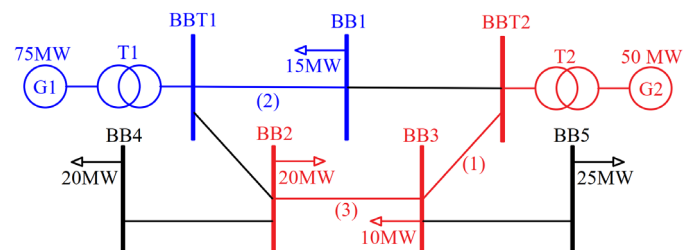
Fig. 6. Example of power system with suboptimal transmission line connections (blue color for G1 and red color for G2)
