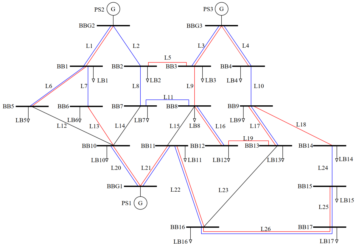
Fig. 10. Simulation results: lines connected as a result of simulations for the algorithm presented in paper [6] (red lines); lines connected as a result of simulations for p_1 = 1 , p_2 = 0 , and p_3 = 0 (blue lines); lines not connected in any of previously mentioned simulations (black lines)
