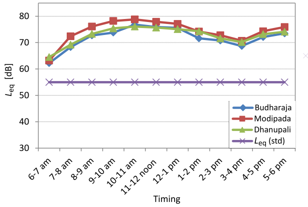
Fig. 4. L_{eq} at different locations (of residential area) during day hours.
