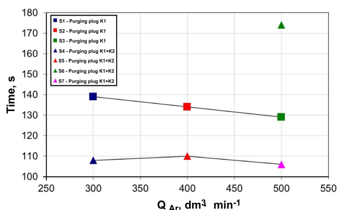
Fig. 10. The numerically determined mixing time required to achieve 95% chemical homogenization of the metal bath, depending on the flow rate of argon injection, for different work configurations purging plugs
