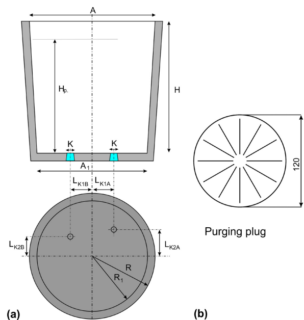
Fig. 1. Geometry of the studied industrial ladle
