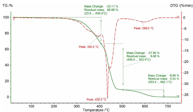
Fig. 5. TG and DTG curves of uncured sample
