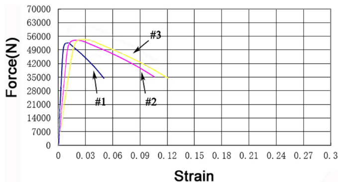
Fig. 2. Force-strain curve of 18Ni (250)
