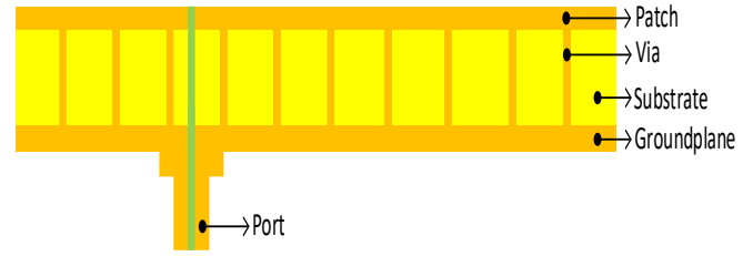
Fig. 2. Side view of U-slotted SIW antenna
