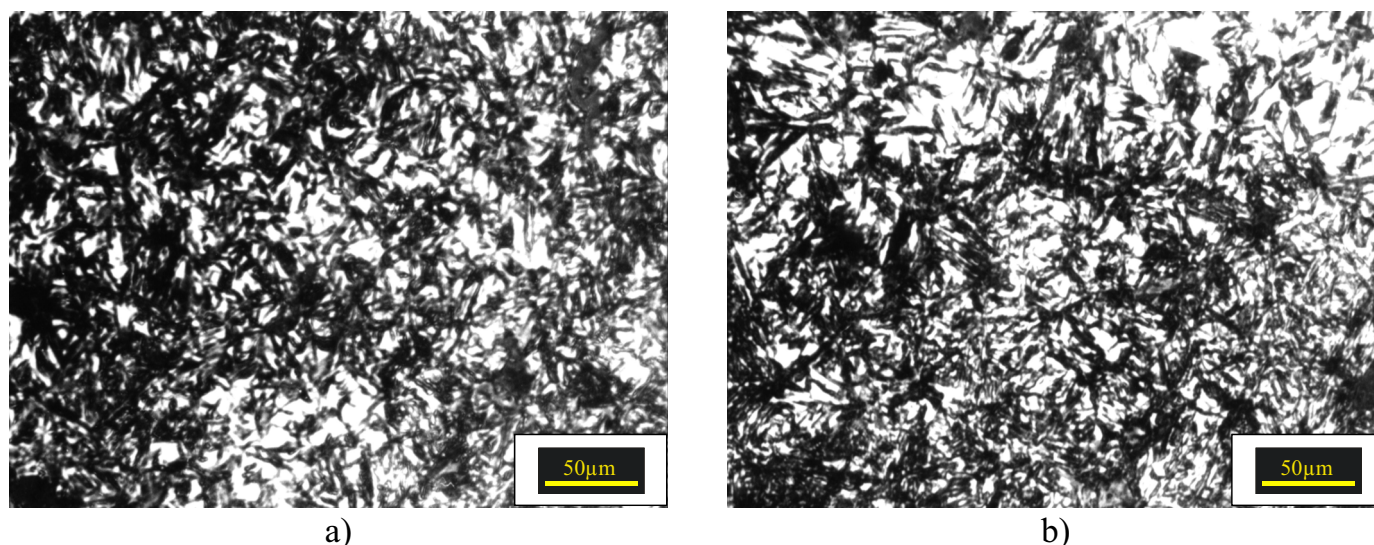
Fig. 2. Photomicrograph of Fe-3%Mn-0.8%C PM steels ATM = 100% H 2 , DP = -60°C [34]: a) 1120°C, SH; bainite, martensite and retained austenite, b) 1250°C, SH; bainite, martensite and retained austenite
