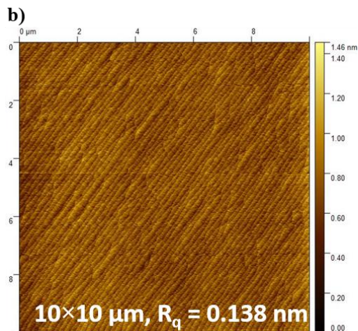
Fig. 12. AFM images of surface of InP:Fe layer deposited at optimal conditions. Roughness R_q = 0.145 nm.
