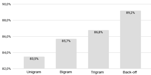
Fig. 8. The quality of prediction of any text on different models for 4 keys of distribution
