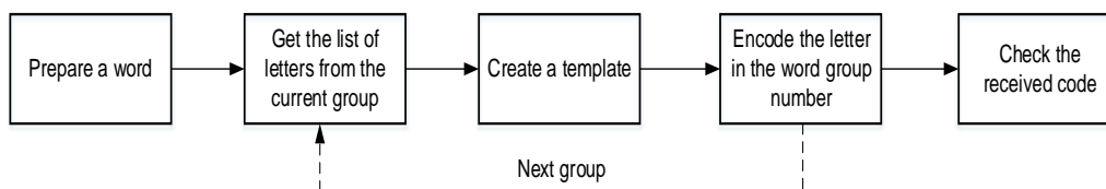
Fig. 5. Word coding diagram
