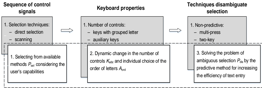
Fig. 4. Diagram the improvement of the method of entering text information with a limited number of control signals
