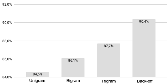
Fig. 9. The quality prediction of any text on different models for the 6-key distribution keys
