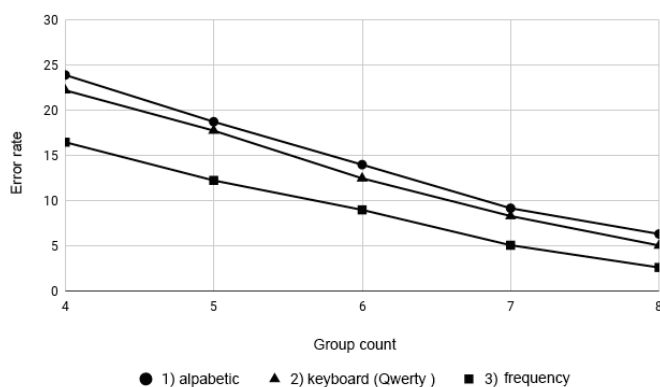
Fig. 6. Error rate for different sequence of letters
