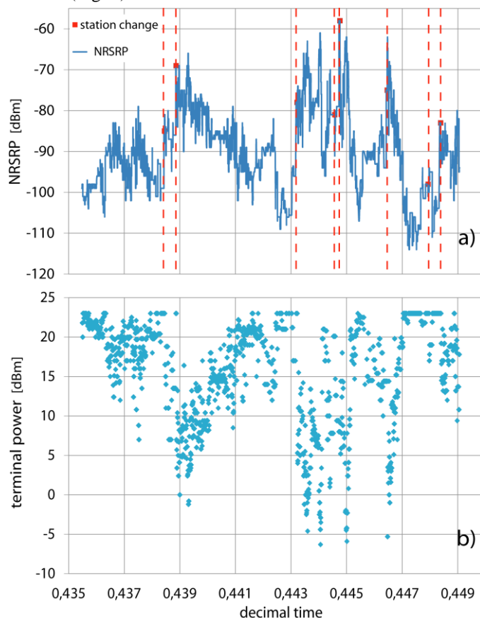
Fig. 15. Measurement results on the route in Piaseczno as a function of decimal time. a) NRSRP received signal level, b) NB-IoT terminal power
