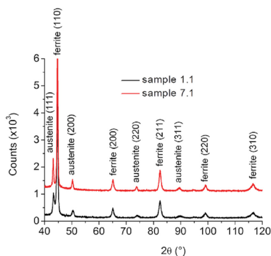
Fig. 3. XRD diffractograms of the sample 1.1 and 7.1 after polishing
