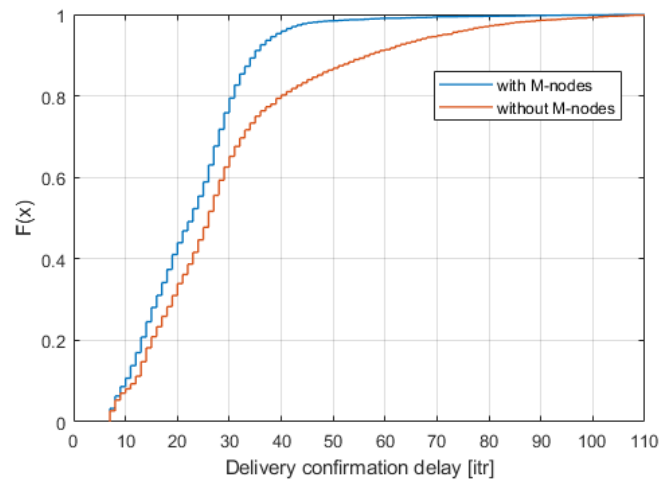
Fig. 2. Distribution of delivery confirmation delay
