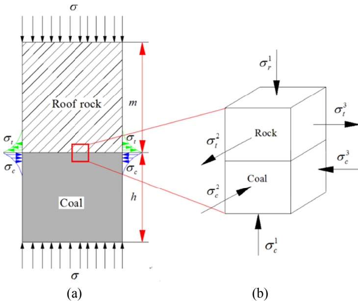
Fig. 2. Mechanical model of RRC composite sample
