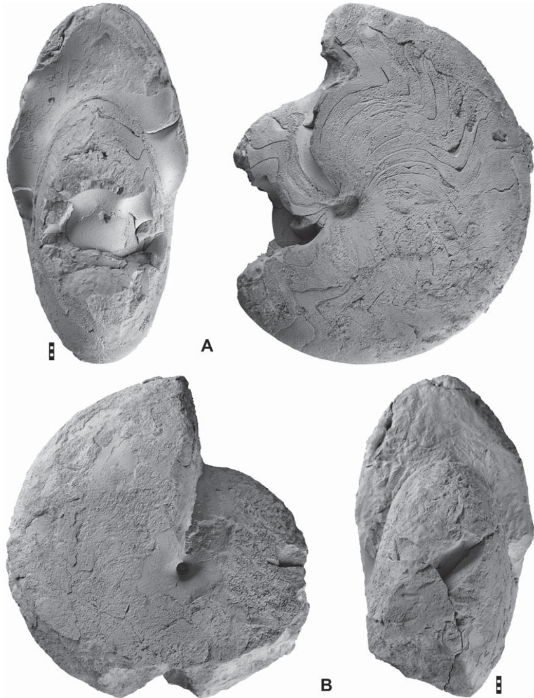
Text-fig. 17. Iranoceras pingue (Walliser, 1966) from Kal-e-Sardar-NW, Iran. A – Specimen MB.C.26860; B – Specimen MB.C.26873. Scale bar units = 1 mm
