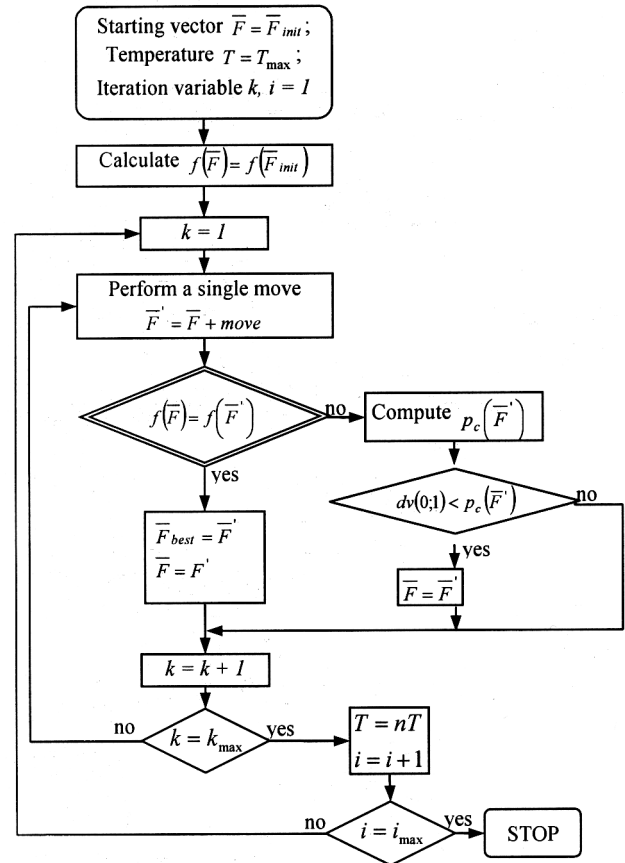
Fig. 10. Simulated Annealing workflow
