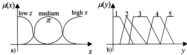
Fig. 8. The membership functions: a) of an input LV, b) of output LV
